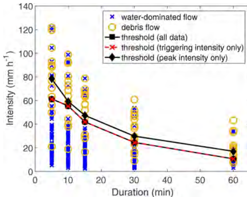
Figure 6.6. Rainfall intensity-duration thresholds to produce water-dominated flow and debris flows in small watersheds following the Buzzard Fire in southwestern NM. The black and red lines represent threshold intensity-duration values for a calibrated model (McGuire and Youberg, 2020).
