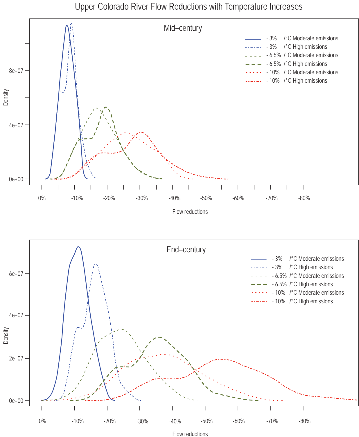
Figure 3.4. Probability of change in the flow in the Upper Colorado River as a function of greenhouse gas emissions and the sensitivity of runoff to temperature, from Udall and Overpeck (2017). The percentages in the legend are percent reduction in runoff per degree Celsius of warming and range from a reasonable lower limit to a reasonable upper limit, with the most likely value (-6.5% per degree) in the middle. The 'moderate emissions' scenario corresponds to SRES A1B/RCP4.5 and the 'high emissions' to SRES A2/RCP8.5.
