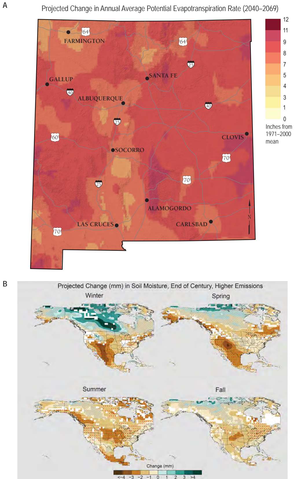
Figure 2.6. (a) Projected change in annual rate of Potential Evapotranspiration (PET) (inches from 1971–2000 mean), derived from the same projections used for Figs. 2.1b and 2.3. (b) Projected changes in seasonal soil moisture by the end of the twenty-first century across North America, adapted from USGCRP (2017).
