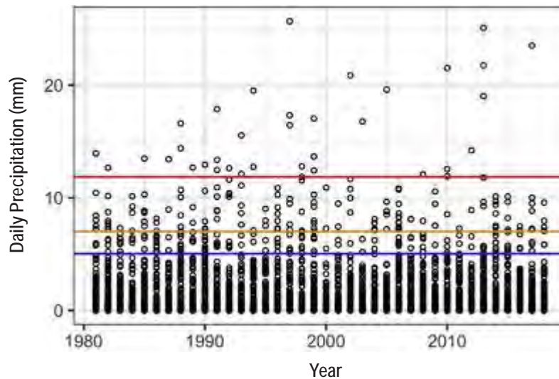
Figure 8.2. Monsoon season (Jul–Sept) daily precipitation across the upper Rio Grande watershed in northern New Mexico from 1981 to 2018 (from Towler et al., 2020). Horizontal lines are select quantiles: Q91 = 5.0 mm/d (0.20 in, blue), Q95 = 7.0 mm (0.28 in, orange), and Q99 = 11.9 mm (0.47 in, red). Thus the most extreme daily precipitation amounts, in the 99th percentile, occur above the red line with amounts >11.9 mm (0.47 in). Towler et al. (2020) used a precipitation threshold of 5 mm/day (0.20 inch/day) to define extreme events.
