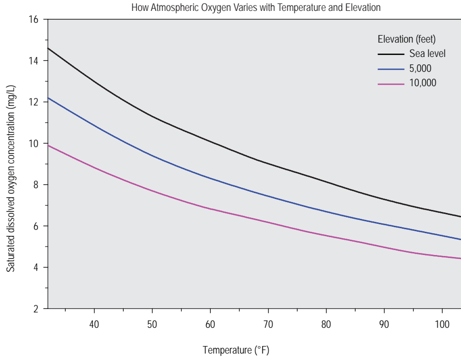
Figure 9.6. Dependence of the saturated dissolved oxygen concentration (mg/L) in equilibrium with the atmosphere on temperature and altitude.
