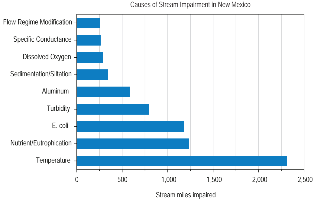
Figure 9.2. Principal causes of surface-water impairment of streams and rivers (NMED, 2021a).
