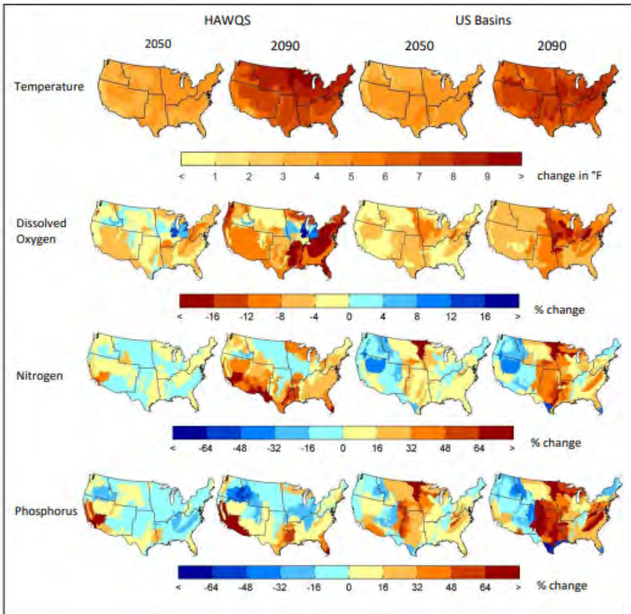
Figure 9.5. The effects of climate change in water-quality parameters under RCP8.5 in 2050 (2040–2059) and 2090 (2080–2099) relative to the reference period (1986–2005). Results for each eight-digit HUC represent the average values across the five GCMs, and are aggregated to the Level-III Ecoregions (EPA, 2017).
