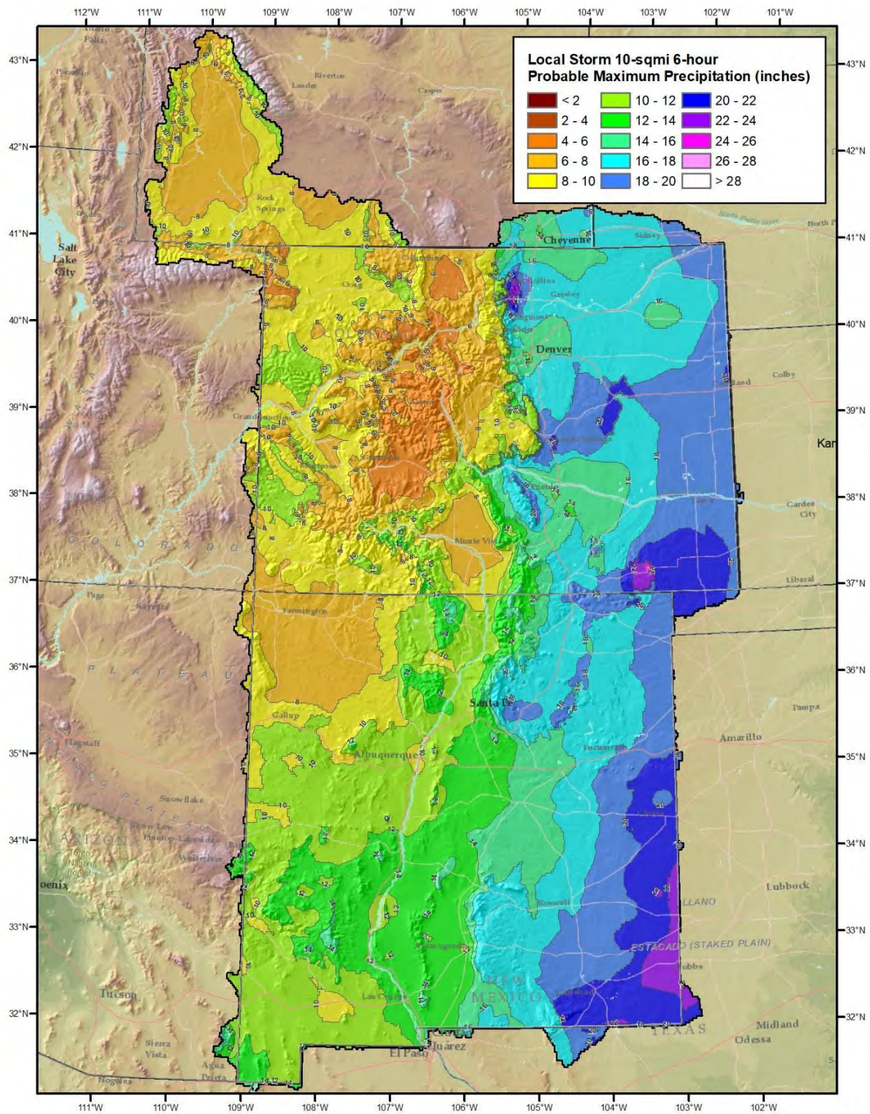
Figure 8.5. Probable maximum precipitation (PMP) for a local storm (10 square miles) of 6-hour duration (CO DWR and NM OSE, 2018).
