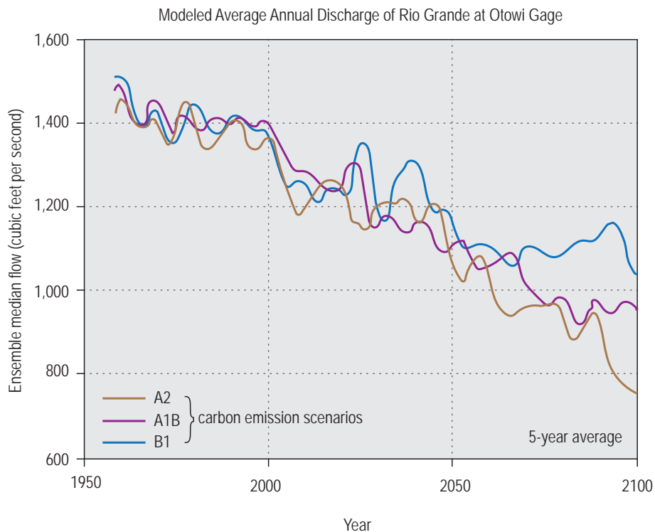
Figure 3.3. Modeled 5-year average discharge of the Rio Grande at the Otowi gage, in cubic feet per second, from 1950 to 2100 (Llewellyn and Vaddey, 2013). A2 represents high, A1B represents moderate, and B1 represents low carbon emission scenarios.
