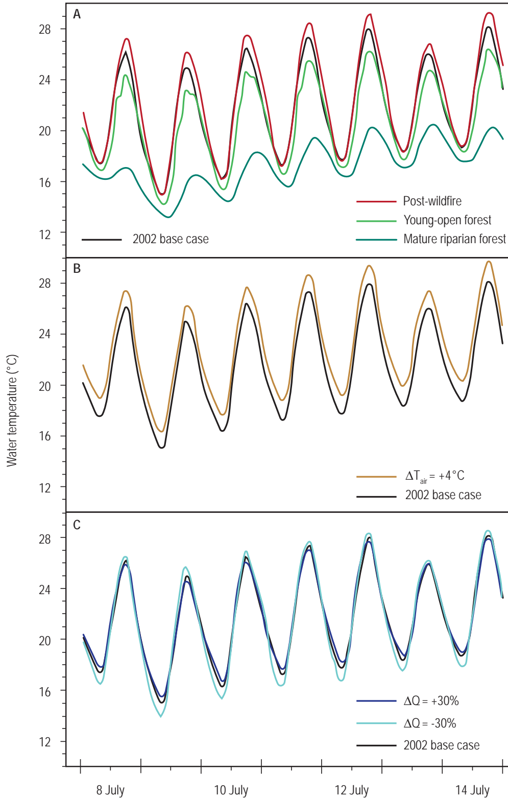
Figure 9.7. Hourly stream temperature time series at RKM 14.05 for the seven-day period over which the heat budget is summarized (from Wondzell et al., 2019, fig. 3). (a) Four riparian vegetation scenarios with 2002 base-case conditions for air temperature ( T_{air} ) and discharge ( Q ). (b) Two air temperature scenarios with 2002 base-case conditions for riparian vegetation and Q . (c) Three discharge scenarios with 2002 base-case conditions for riparian vegetation and T_{air} .
