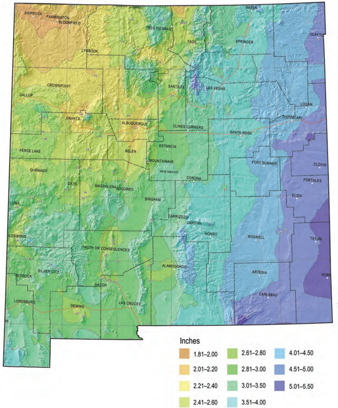
Figure 8.1. Map of rainfall depth produced by 100-year, 6-hour storms in New Mexico (NWS, 2005a).
