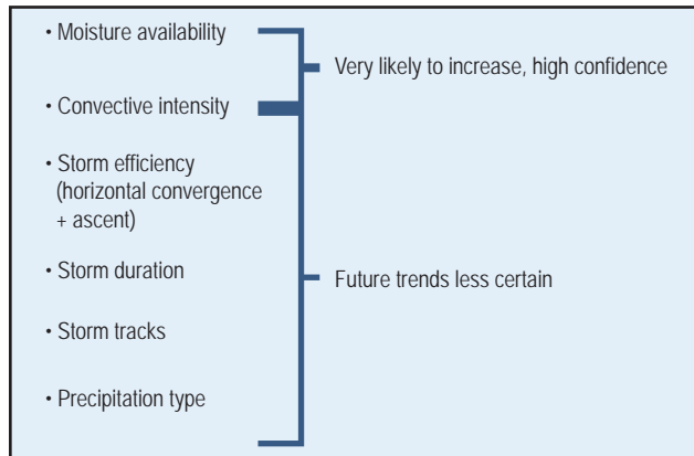
Figure 8.3. The principal mechanisms that may increase precipitation from PMP events and summary of current confidence in future changes of these mechanisms (McCormick et al., 2020).
