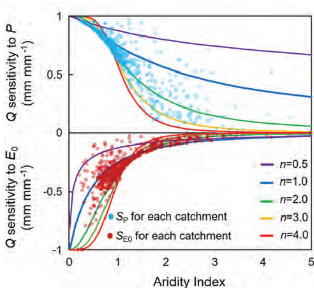
Figure 10.1. Sensitivity of Q (runoff + recharge) to changes in the aridity index ( E_0/P ), from Yang et al. (2018). High values of the aridity index correspond to arid climate and low values to humid climate. P is precipitation and E_0 is potential evapotranspiration (both with units of mm/yr). 'n' is a factor that accounts for the effects of processes other than P and E_0 on runoff + recharge, such as seasonality or intensity of precipitation. The red and blue dots are empirical data for change in Q as a function of change in P and E_0 , from 1981 to 2010, from 710 drainage basins worldwide. They indicate the number of mm/yr that Q changed in response to a 1 mm/yr change in P or E_0 . The distribution of the data points indicates that 'n' typically varies between 1 and 3 and averages about 2.
