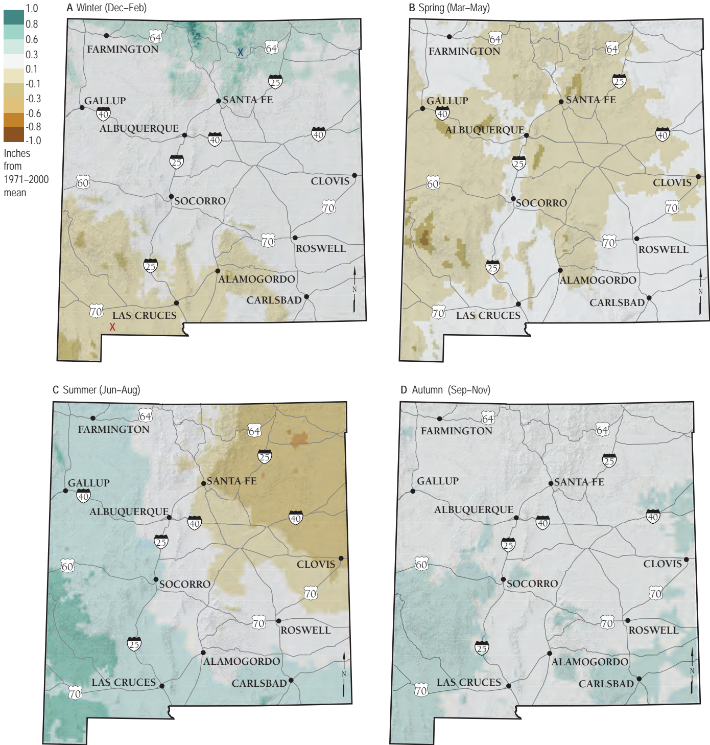
Figure 2.3. Seasonal average precipitation changes simulated by the same ensemble of climate simulations used for Fig. 2.1. (a) winter (b) spring (c) summer (d) autumn. As in Fig. 2.1a, each map shows differences between two thirty-year averaging periods 70 years apart: (2040–2069) minus (1971–2000). The color scheme is the same for each plot, with green colors indicating increasing precipitation and brown colors indicating decreasing precipitation. In panel (a), the blue and red x symbols denote the locations associated with time series shown in Fig. 2.4.
