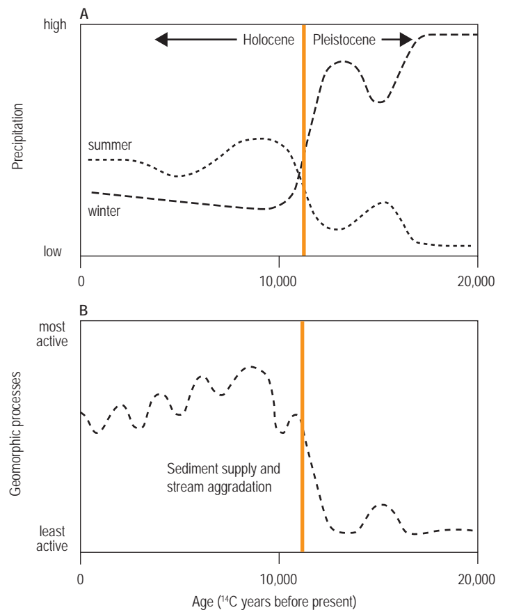
Figure 6.2. Graph showing geomorphic processes active in the Pajarito Plateau with time (in years before present from carbon-14 dating) and precipitation. Adapted from Reneau (1996). Panel A shows the precipitation regime changing from a winter precipitation (snow) dominated regime to a summer precipitation regime at the Pleistocene/Holocene boundary approximately 11,700 years before present. Panel B shows the increases in geomorphic processes, including sediment being supplied to the canyon stream channels that coincides with the change in precipitation regime at the Pleistocene/Holocene boundary.
