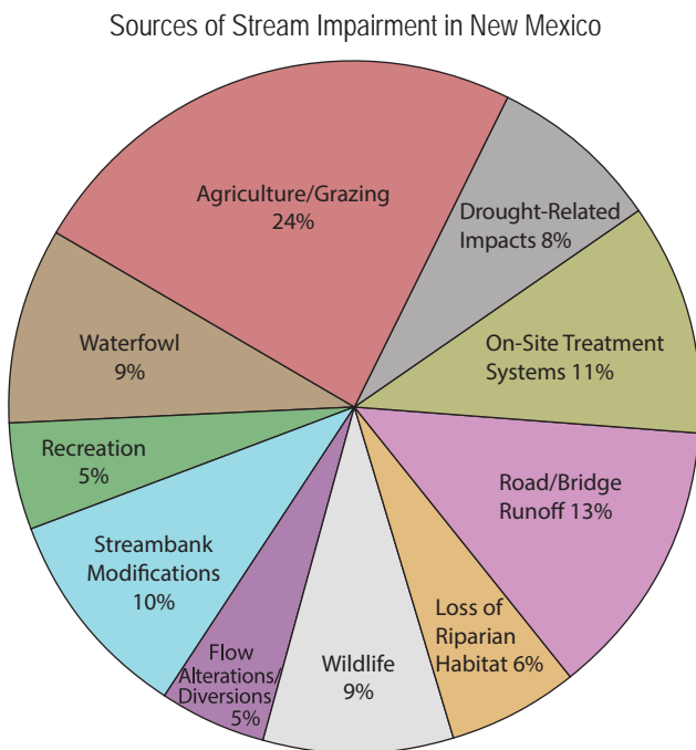
Figure 9.4. Probable sources of surface-water impairment in streams and rivers of New Mexico as reported in approved TMDLs (NMED, 2021a).
