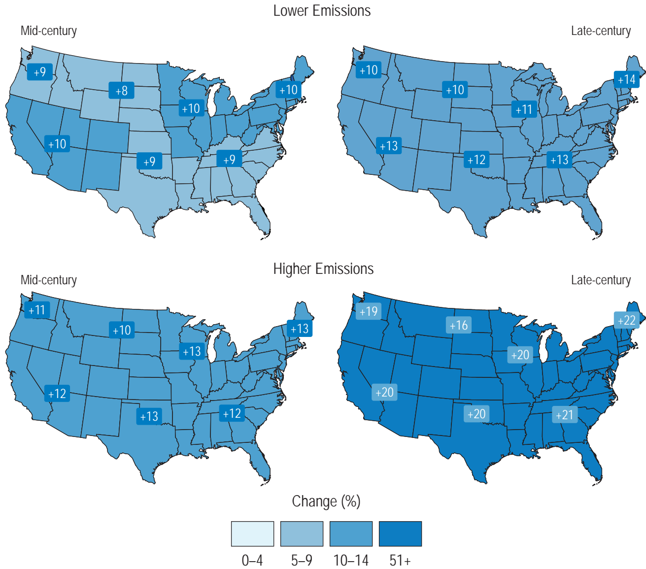
Figure 2.5. Projected change from a historical baseline period (1901–2005) in the magnitude of extreme precipitation events, here defined as the one-day precipitation maximum expected once every 20 years, derived from statistically downscaled CMIP5 GCM simulations (using an average of CMIP5 models, but a different statistical downscaling technique than the MACA post-processing used for Figs. 2.1–2.4; USGCRP, 2017, Fig. 7.7). Results from a lower emissions scenario (RCP 4.5) are on the top; higher scenario results (RCP8.5) are on the bottom. The left-side maps show changes as a percentage of present-day 20-year return values expected by mid-century; late-twenty-first century changes are shown on the right. All changes projected nationwide are positive, indicative of higher 20-year return values of maximum daily precipitation.
