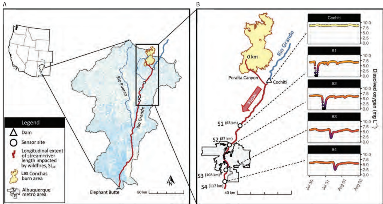
Figure 9.10. Summary of impacts of Las Conchas fire on dissolved oxygen concentrations in the Rio Grande (Ball et al., 2021).
